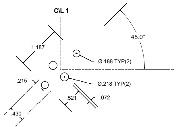
-2 HOLE PATTERN 2:1 SCALE
